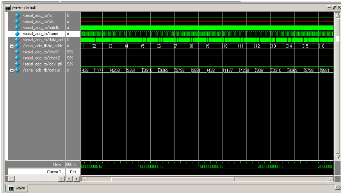
Figure 3 - Post-Route Timing Simulation Results Showing a Repeating Data Pattern
