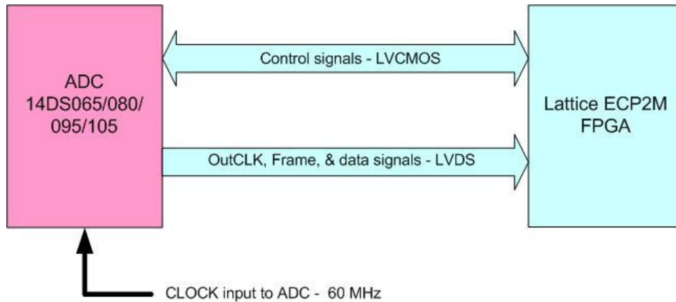
Figure 2 – Block Diagram of Serial ADC Connections to the Lattice FPGA
