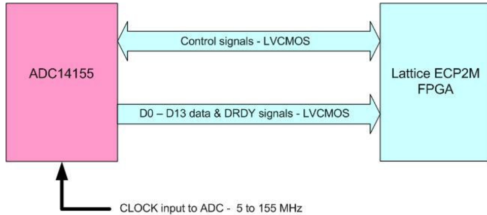
Figure 1 – Block Diagram of ADC Parallel Connections to the Lattice FPGA
