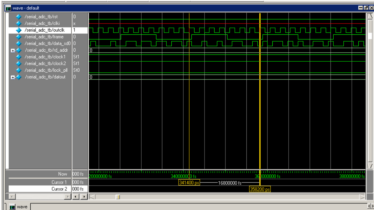
Figure 4 - Post-Route Timing Simulation Results Showing a Data Input Pattern
